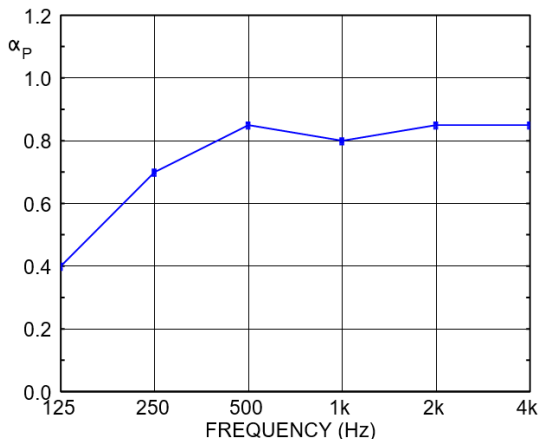
Linea 2.9.10 SOUND ABSORPTION COEFFICIENT MEAN OF 16 MEASUREMENTS
