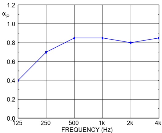
Linea 2.6.8 SOUND ABSORPTION COEFFICIENT MEAN OF 16 MEASUREMENTS
